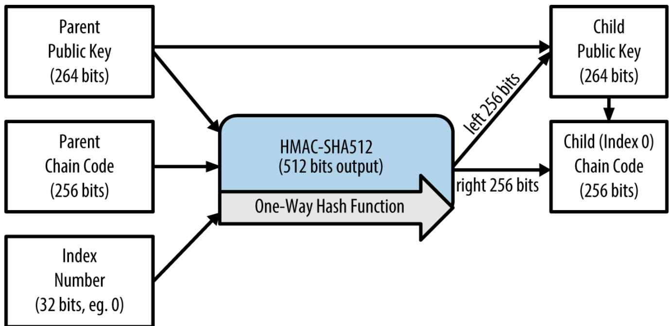
Figure 32. Extending a parent public key to create a child public key
