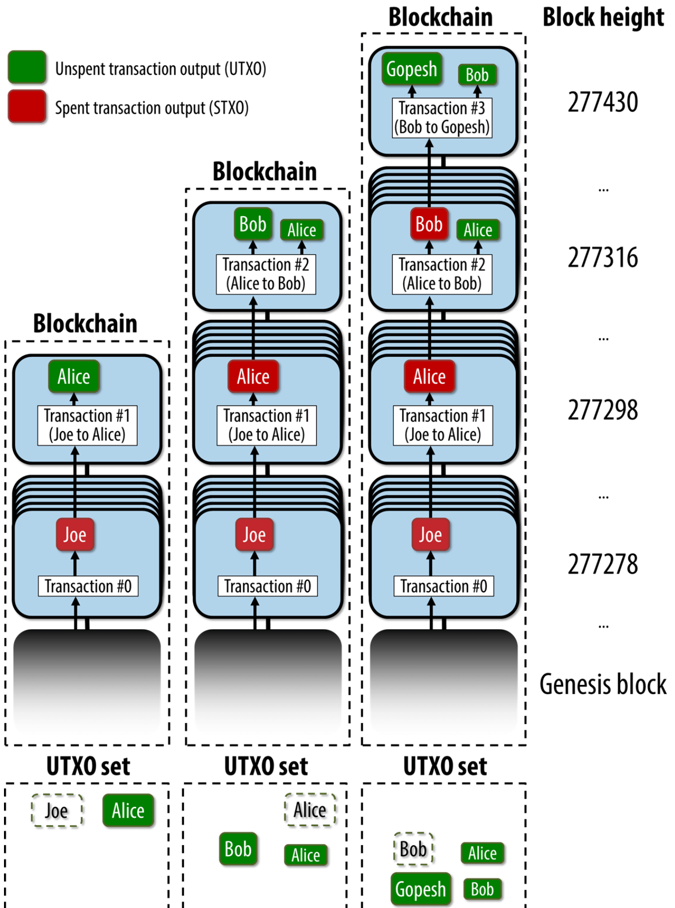
Figure 36. Transaction chain from Joe to Gopesh being built on the blockchain
