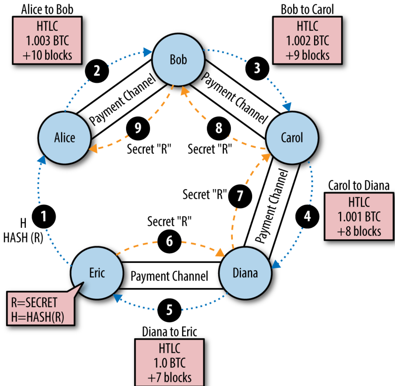
Figure 79. Step-by-step payment routing through a Lightning Network
