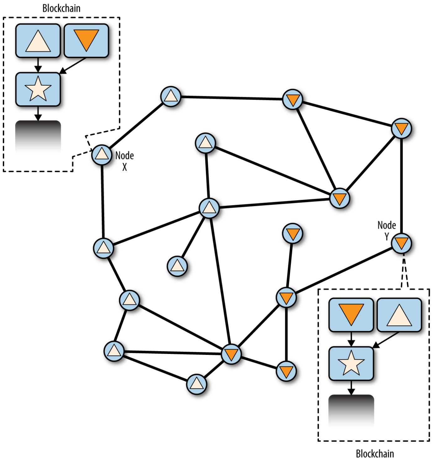
Figure 66. Visualization of a blockchain fork event: two blocks propagate, splitting the network
