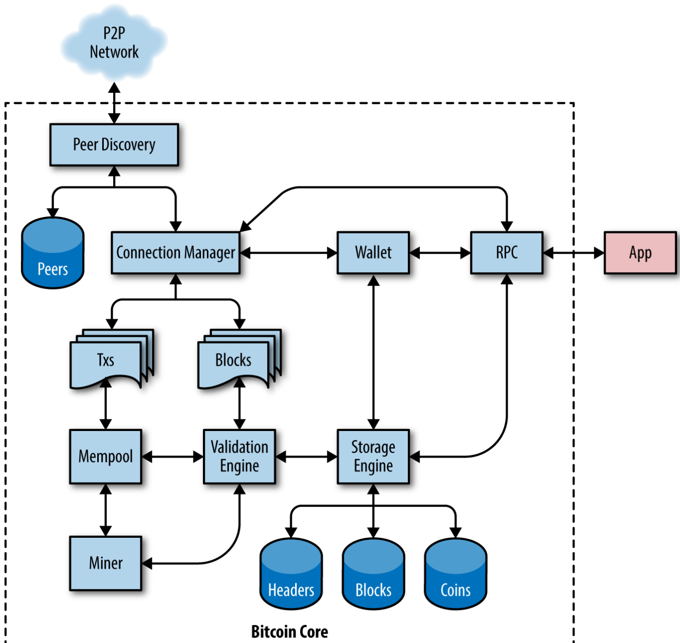
Figure 13. Bitcoin Core architecture (Source: Eric Lombrozo)
