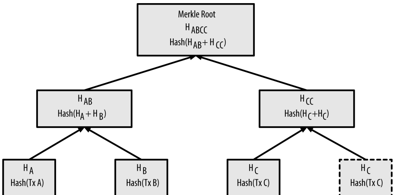
Figure 60. Duplicating one data element achieves an even number of data elements
