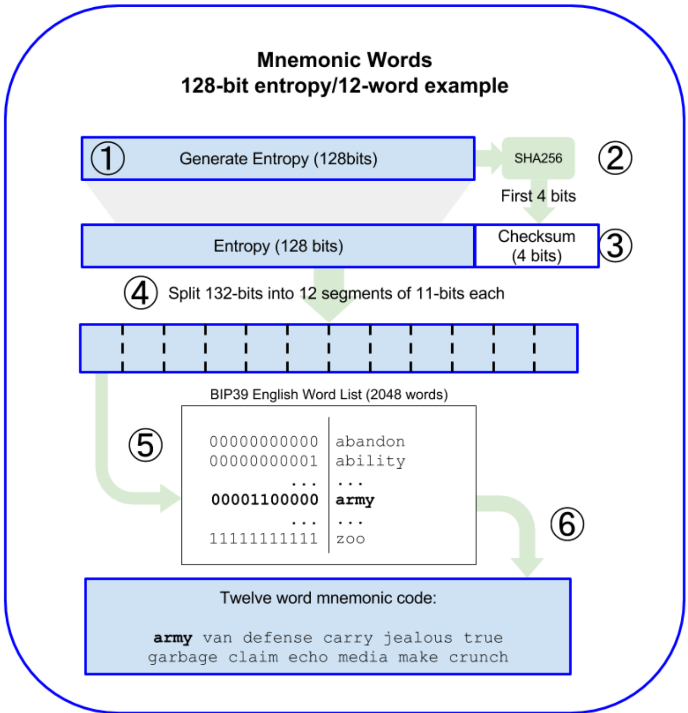
Figure 28. Generating entropy and encoding as mnemonic words
