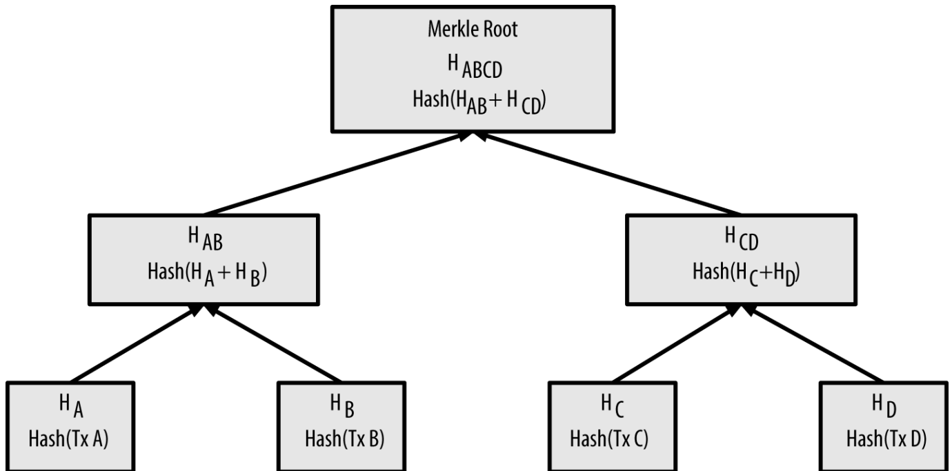
Figure 59. Calculating the nodes in a merkle tree
