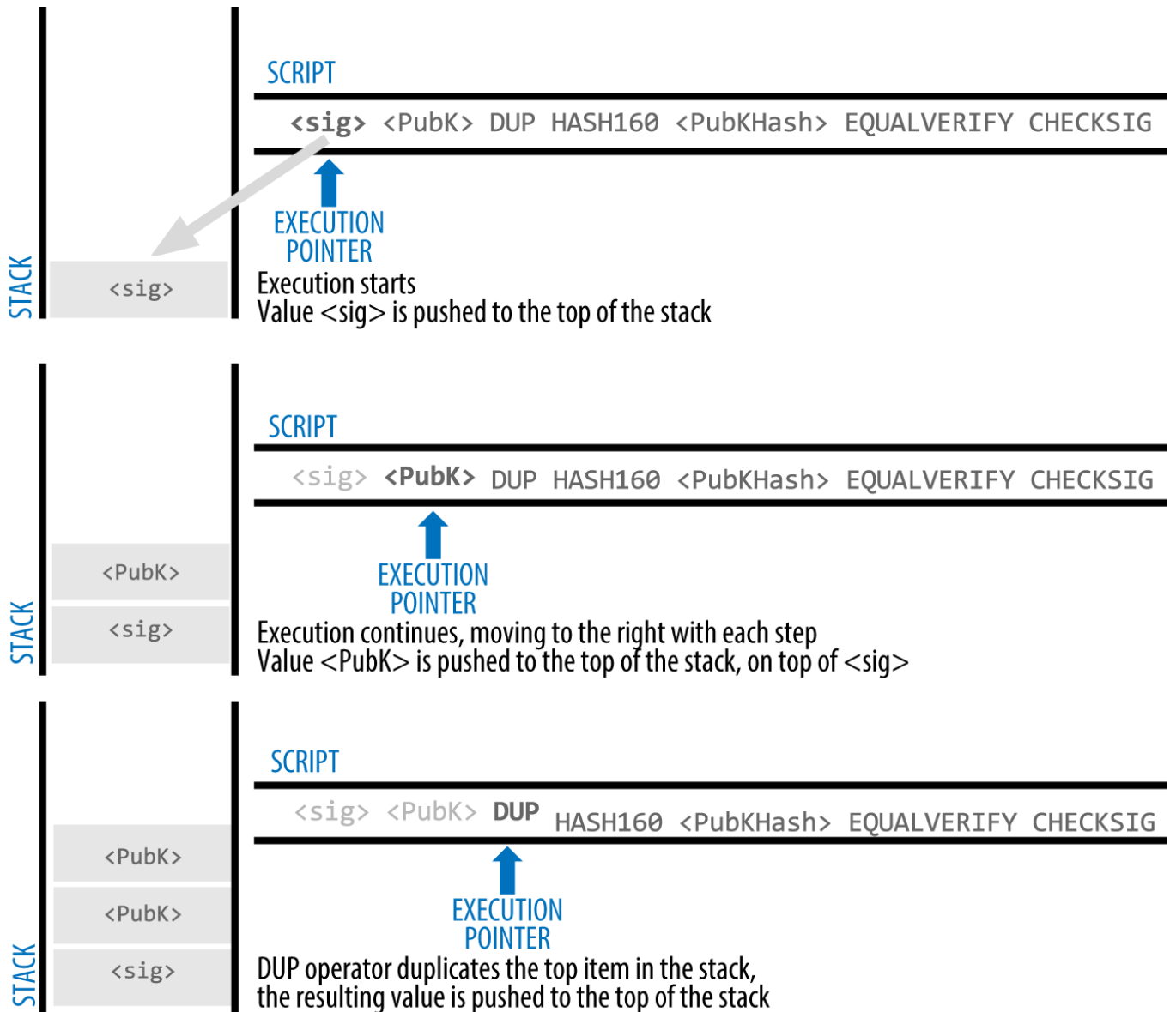
Figure 40. Evaluating a script for a P2PKH transaction (part 1 of 2)
