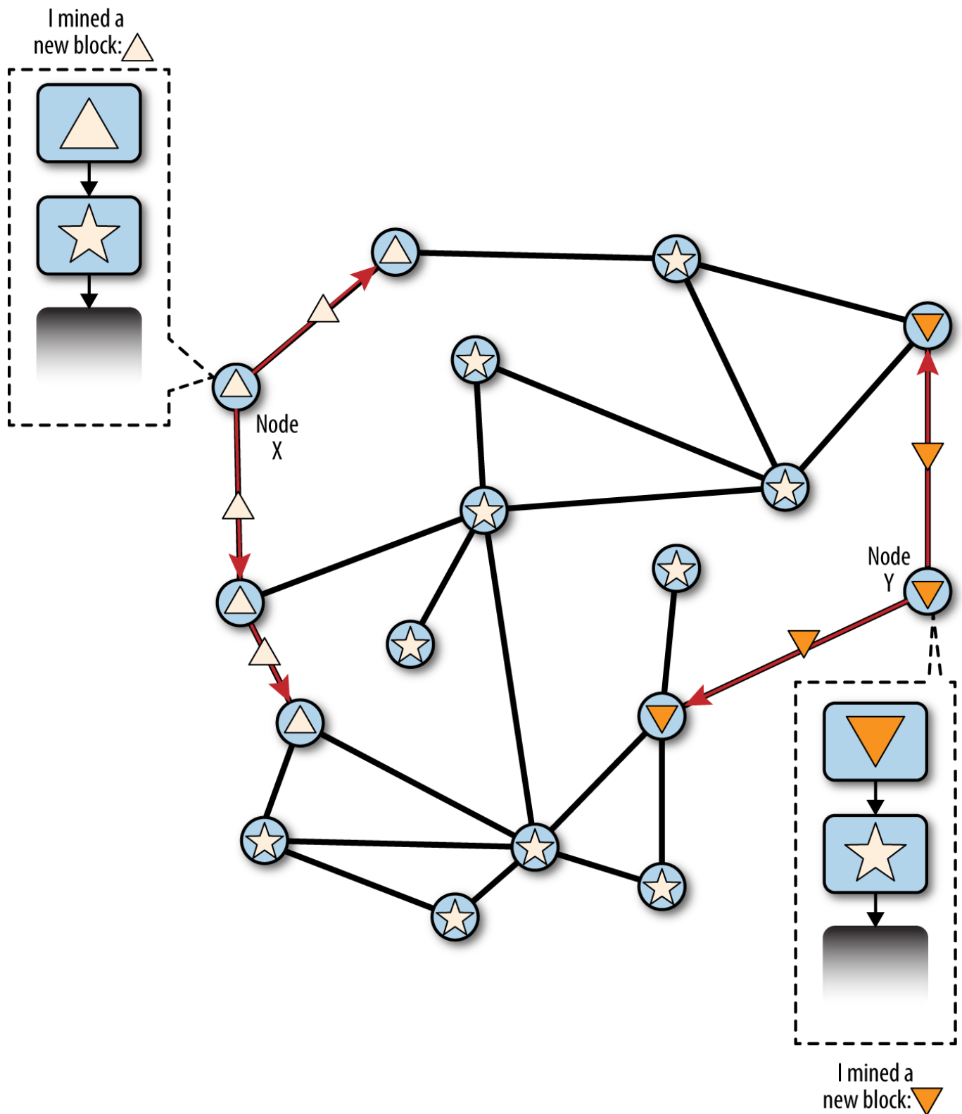
Figure 65. Visualization of a blockchain fork event: two blocks found simultaneously
