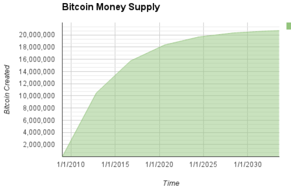
Figure 63. Supply of bitcoin currency over time based on a geometrically decreasing issuance rate
