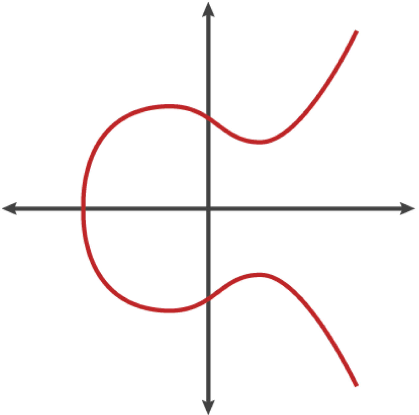
Figure 15. An elliptic curve
