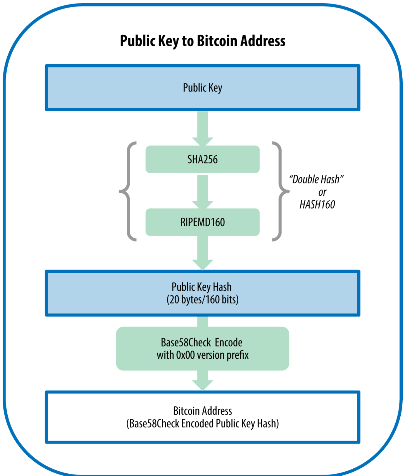
Figure 18. Public key to Bitcoin address: conversion of a public key into a Bitcoin address
