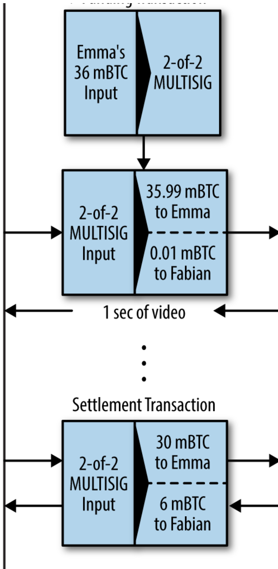
Figure 75. Emma's payment channel with Fabian, showing the commitment transactions that update the balance of the channel
