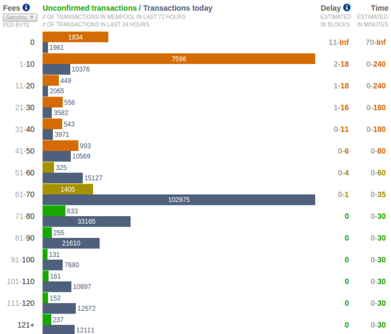
Figure 37. Fee estimation service bitcoinfees.earn.com
