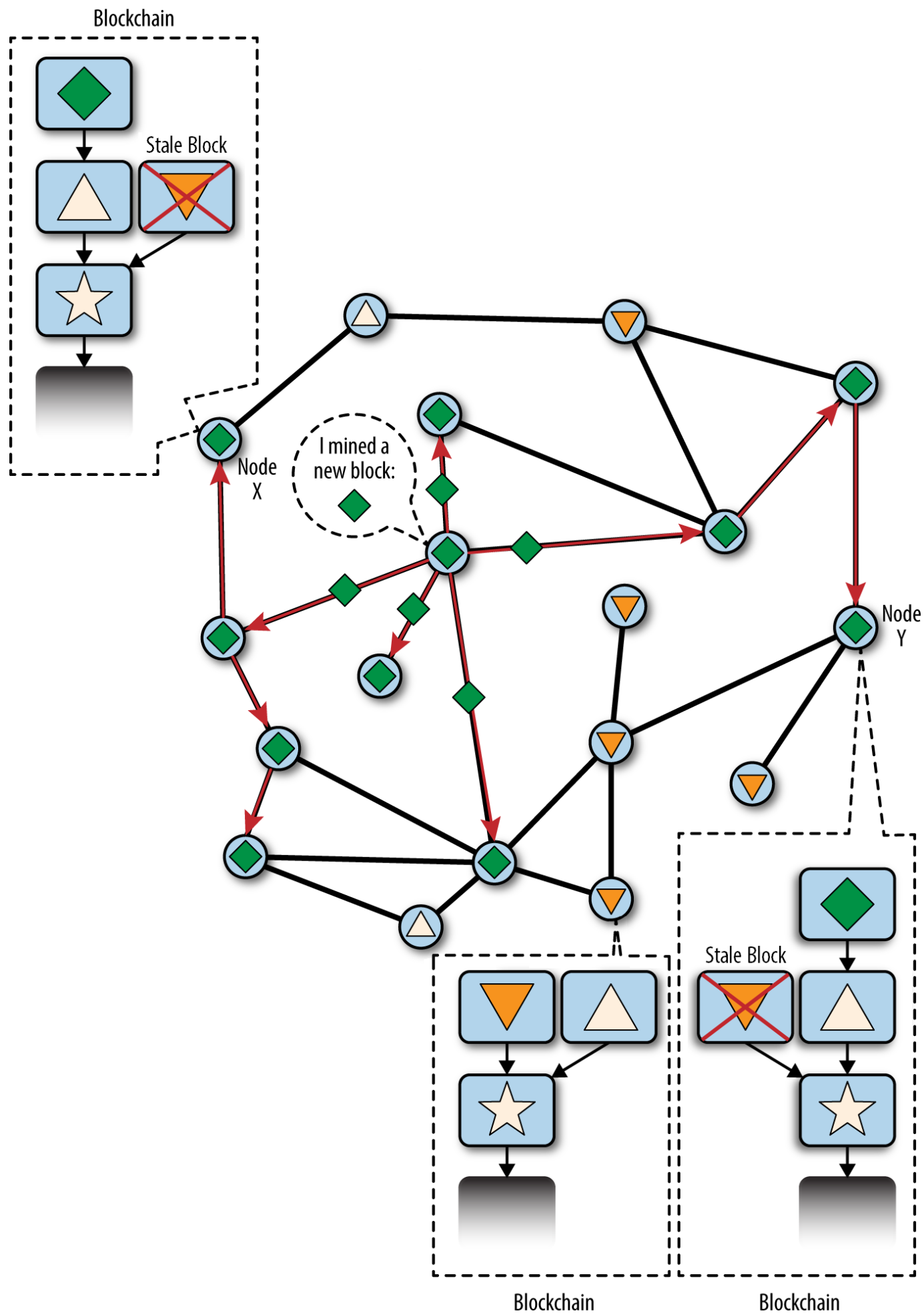
Figure 67. Visualization of a blockchain fork event: a new block extends one fork, reconverging the network. Both Node X and Node Y now consider "upside-down-triangle" block as a stale block.
