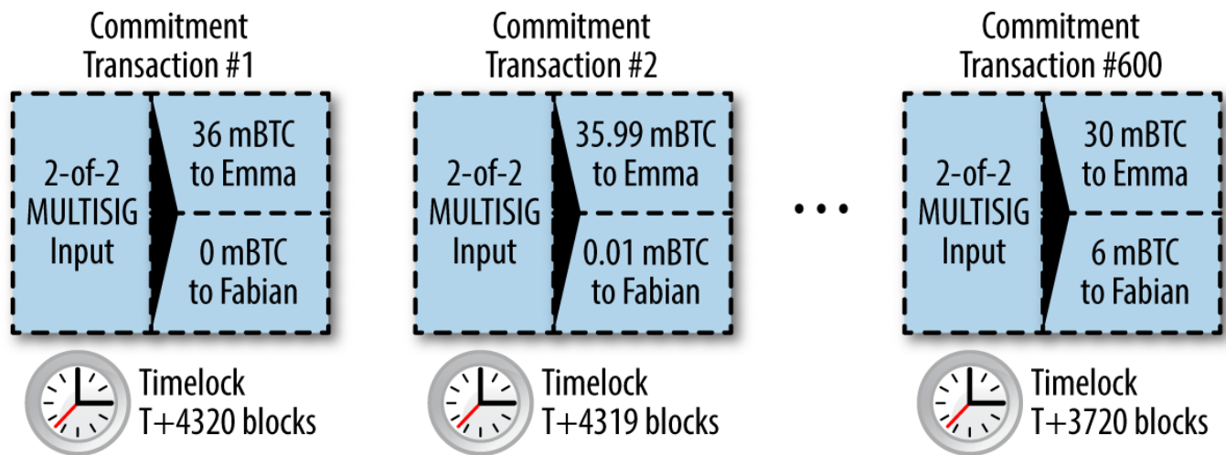
Figure 76. Each commitment sets a shorter timelock, allowing it to be spent before the previous commitments become valid
