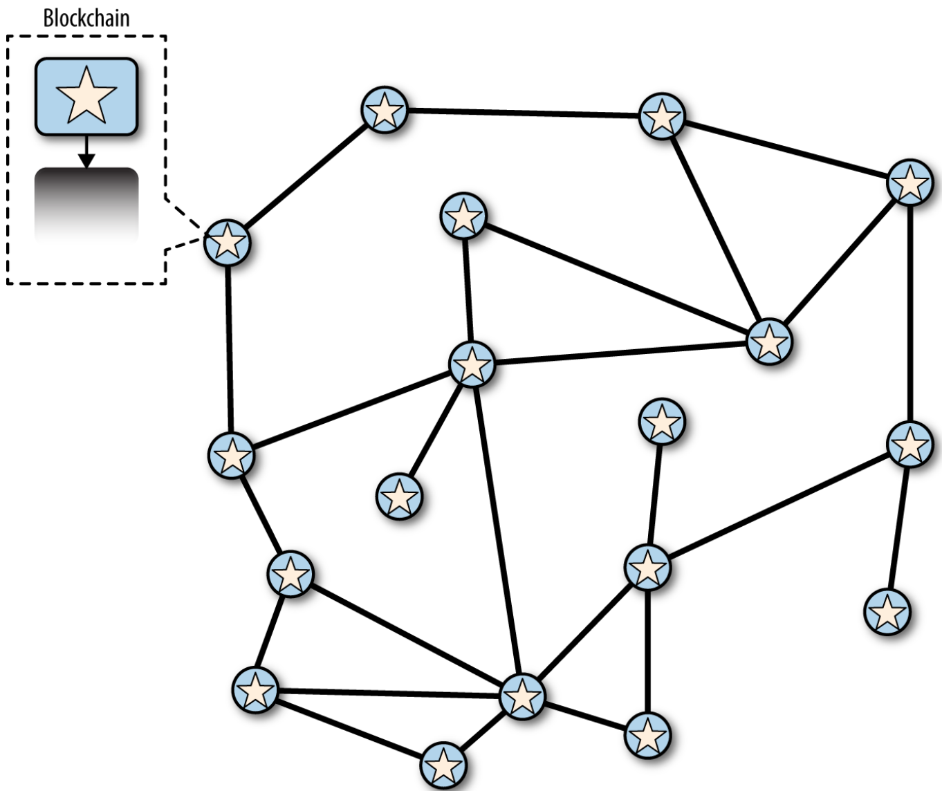
Figure 64. Before the fork—all nodes have the same perspective
