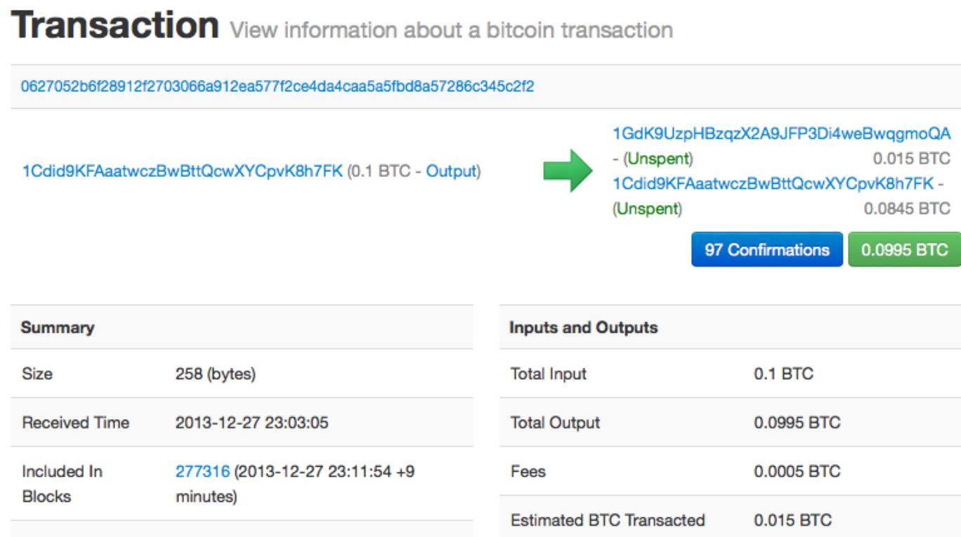
Figure 10. Alice’s transaction to Bob’s Cafe
