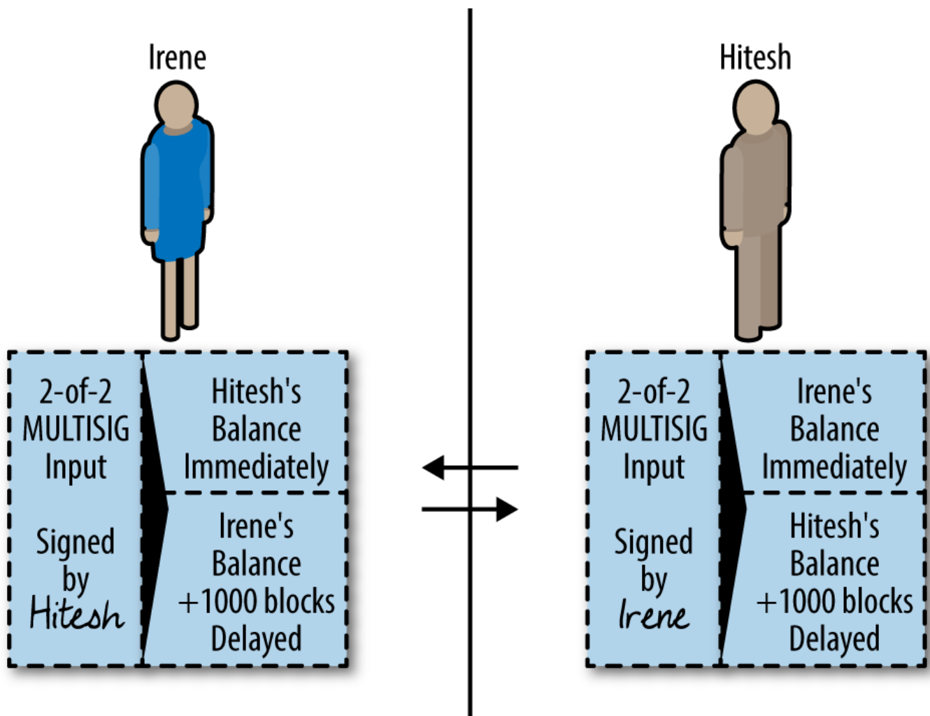
Figure 77. Two asymmetric commitment transactions with delayed payment for the party holding the transaction
