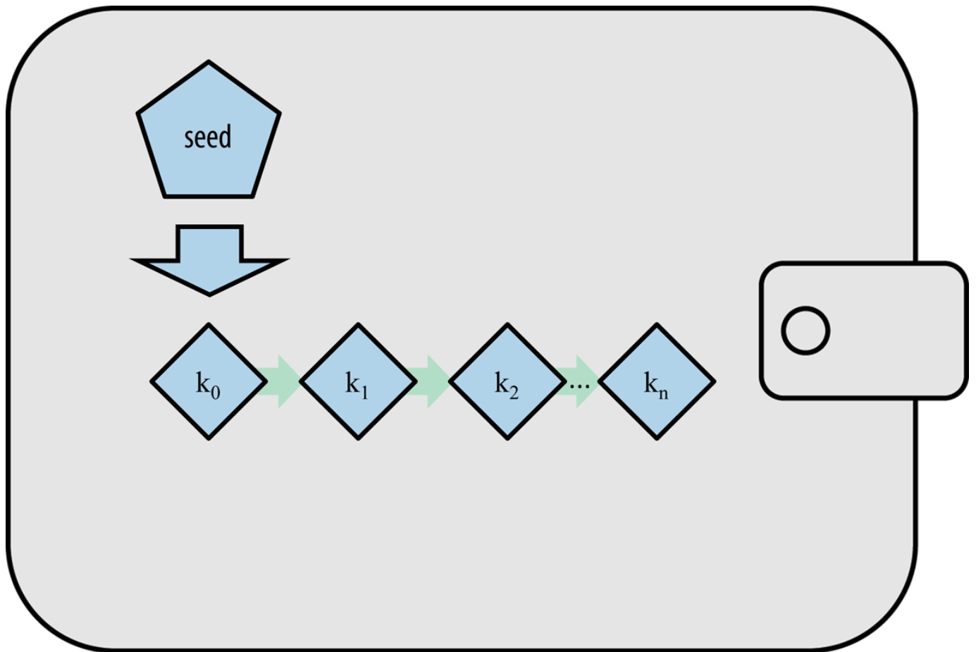
Figure 24. Type-1 deterministic (seeded) wallet: a deterministic sequence of keys derived from a seed
