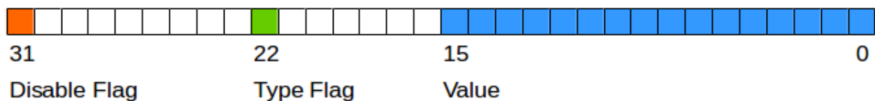
Figure 45. BIP-68 definition of nSequence encoding (Source: BIP-68)
