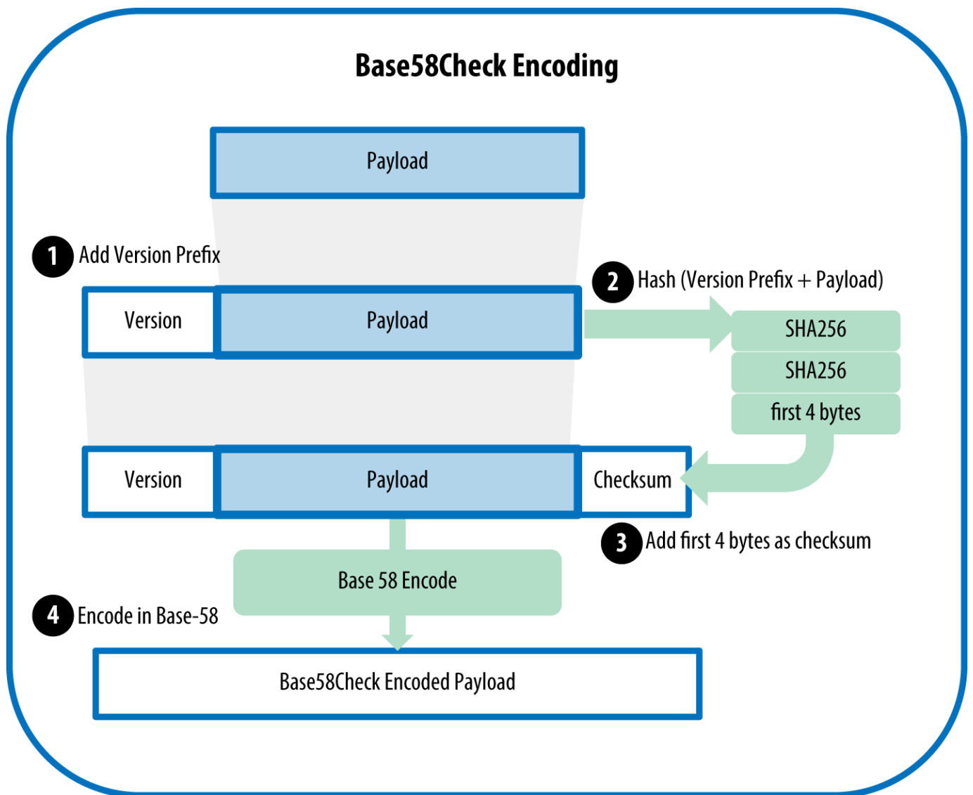
Figure 19. Base58Check encoding: a Base58, versioned, and checksummed format for unambiguously encoding bitcoin data
