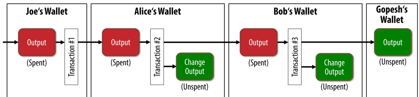
Figure 12. Alice's transaction as part of a transaction chain from Joe to Gopesh, where the output of one transaction is spent as the input of the next transaction
