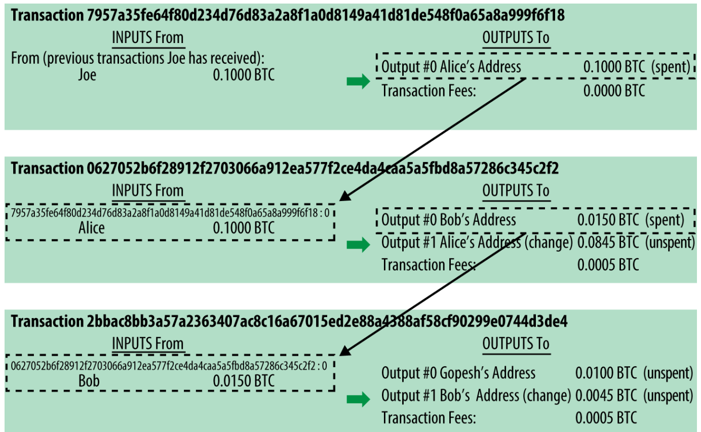
Figure 6. A chain of transactions, where the output of one transaction is the input of the next transaction
