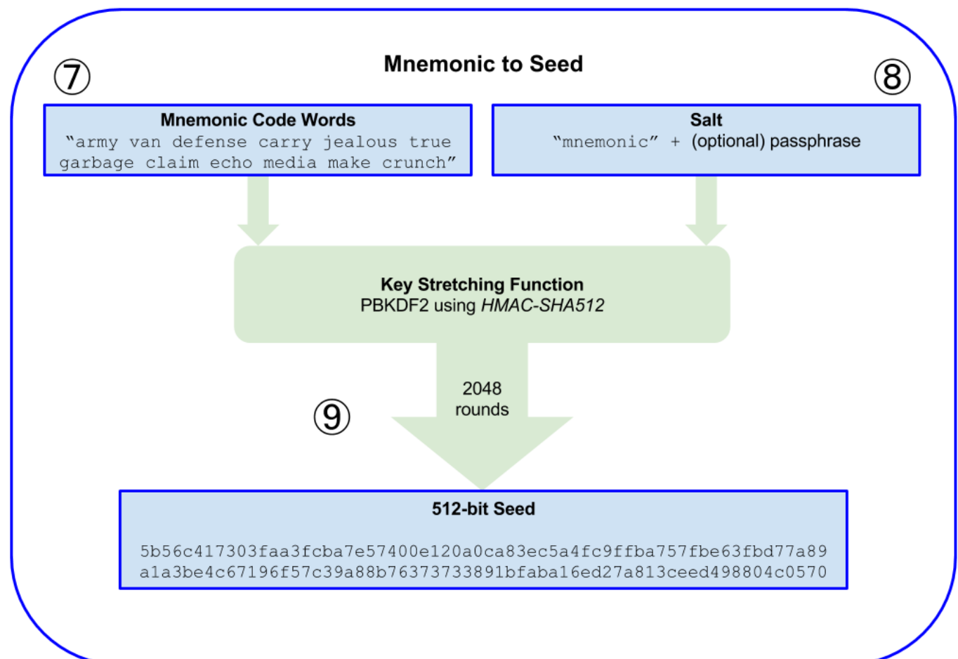
Figure 29. From mnemonic to seed
