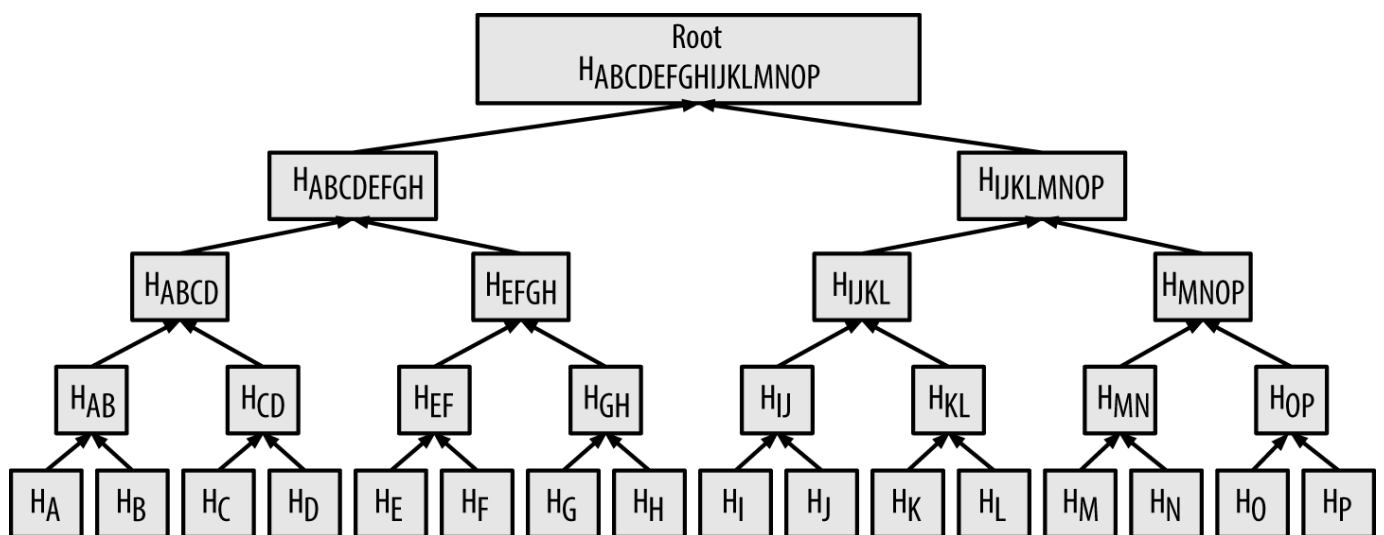
Figure 61. A merkle tree summarizing many data elements
