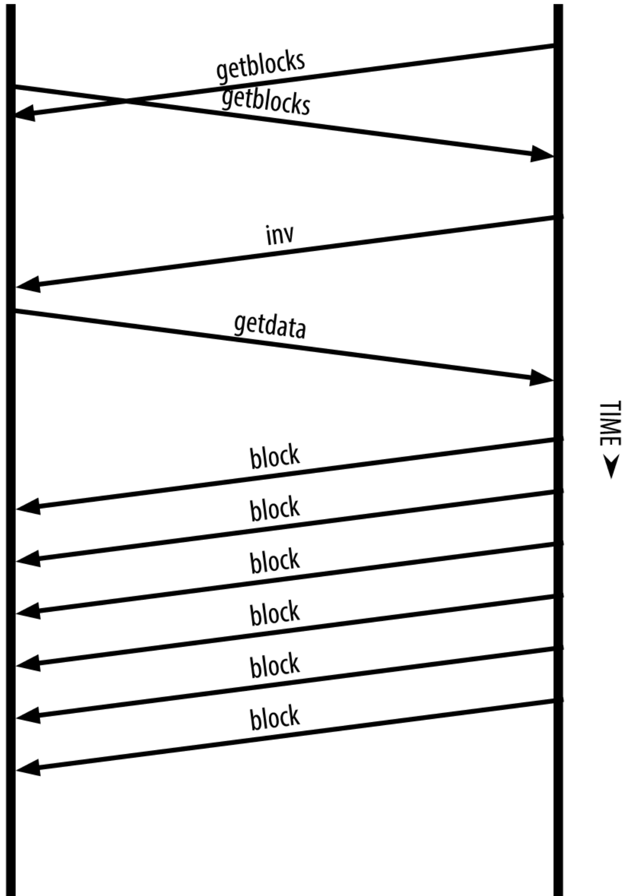
Figure 51. Node synchronizing the blockchain by retrieving blocks from a peer
