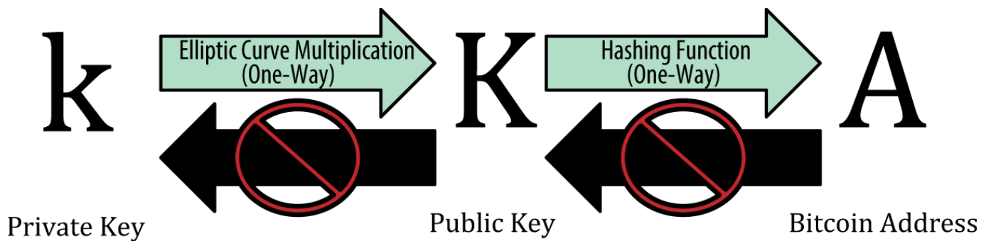
Figure 14. Private key, public key, and Bitcoin address
