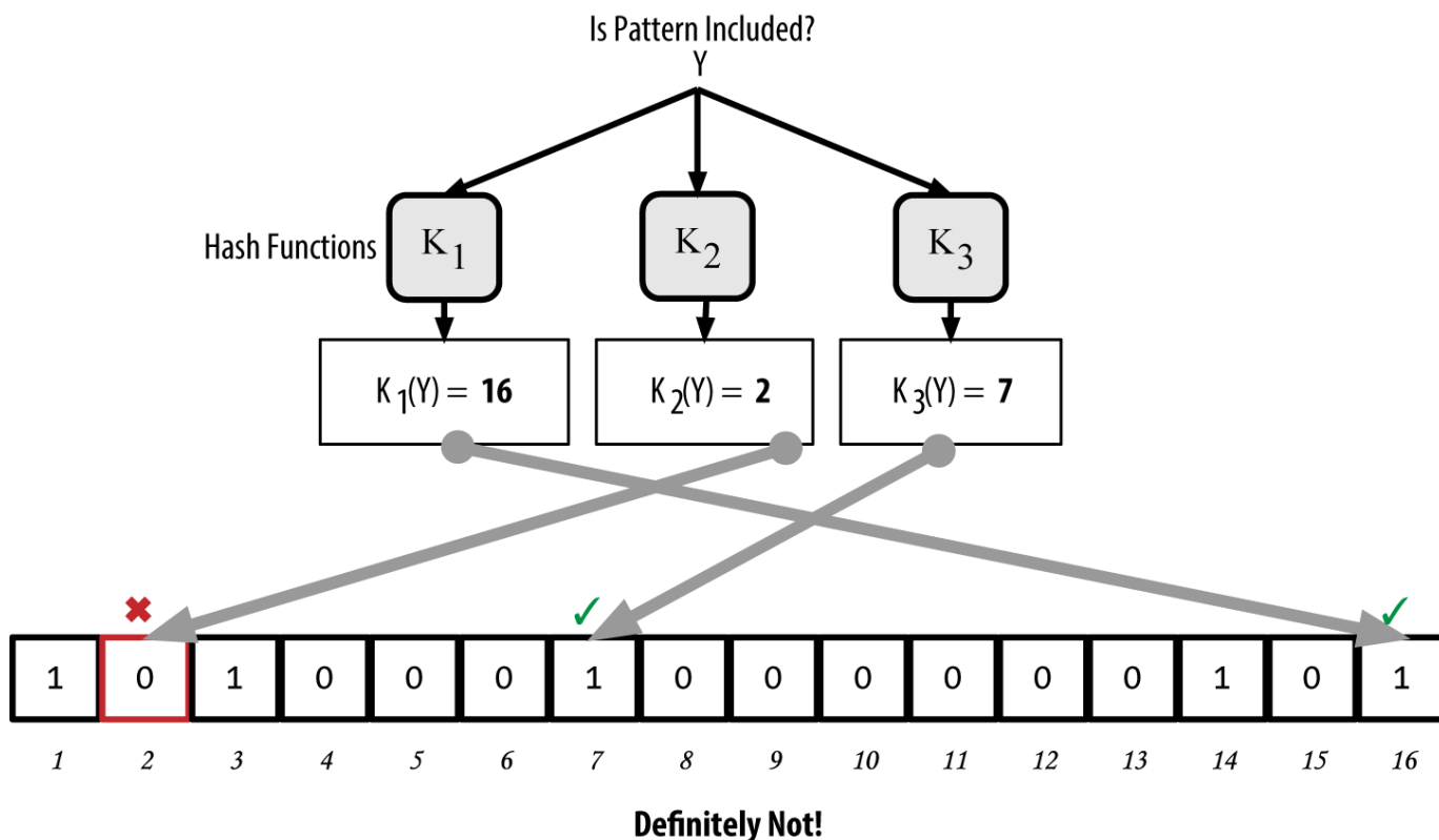
Figure 57. Testing the existence of pattern "Y" in the bloom filter. The result is a definitive negative match, meaning "Definitely Not!"
