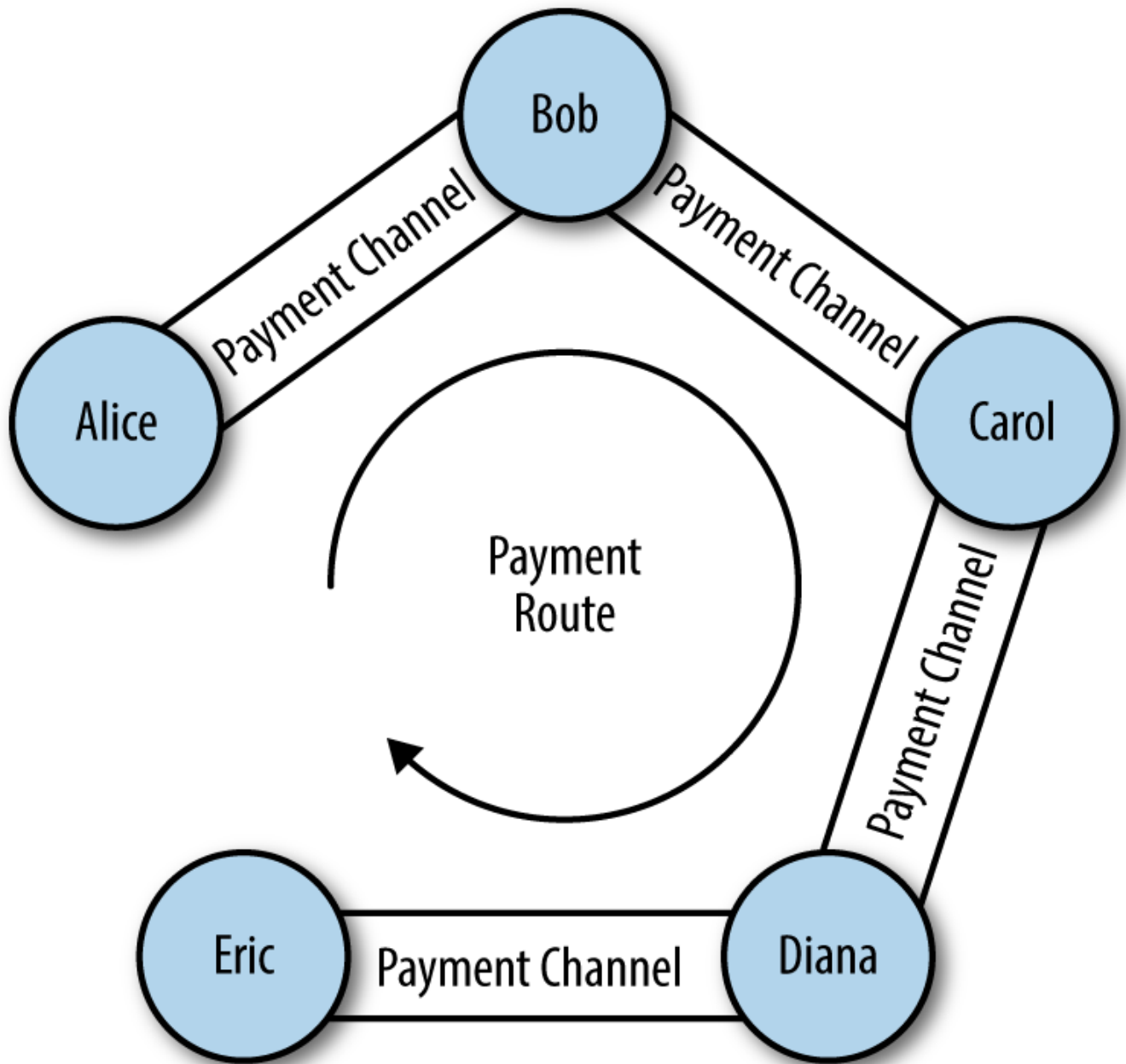
Figure 78. A series of bidirectional payment channels linked to form a Lightning Network that can route a payment from Alice to Eric
