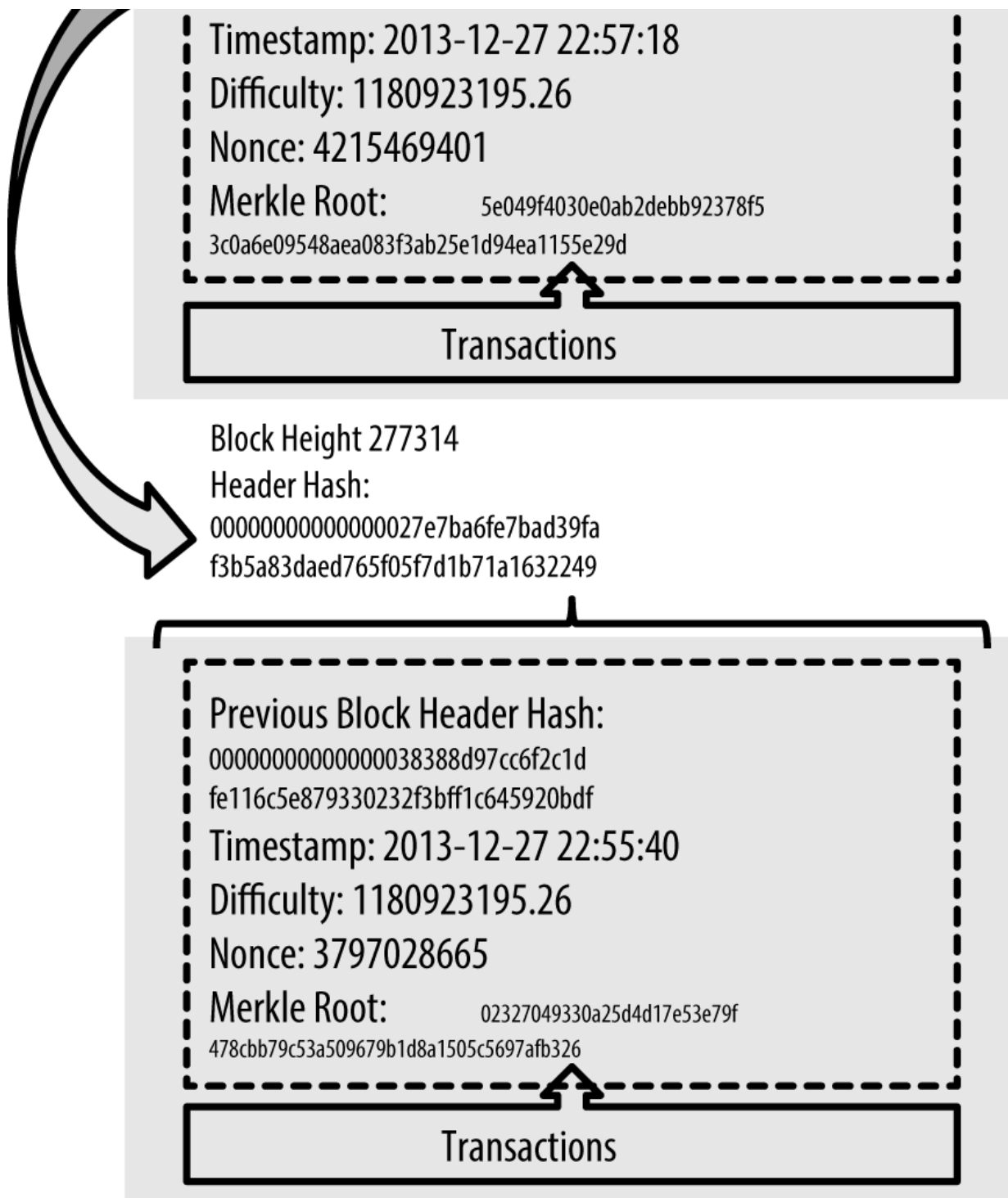
Figure 58. Blocks linked in a chain by reference to the previous block header hash
