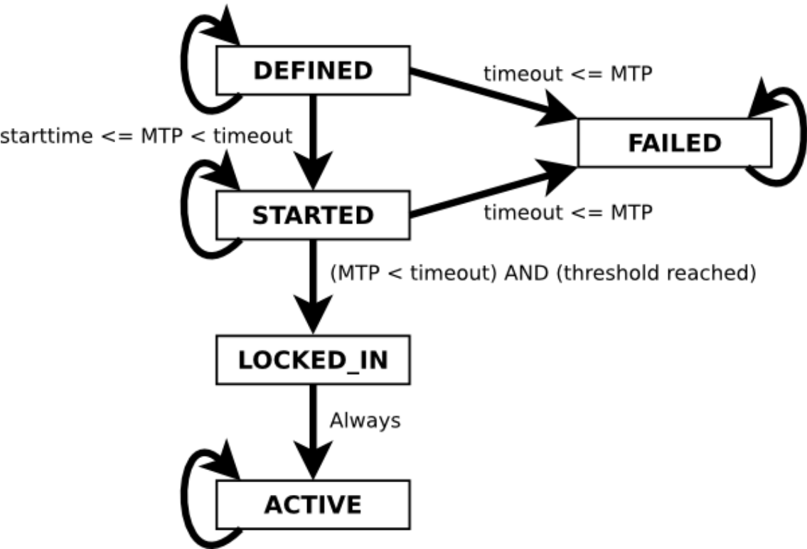
Figure 72. BIP-9 state transition diagram
