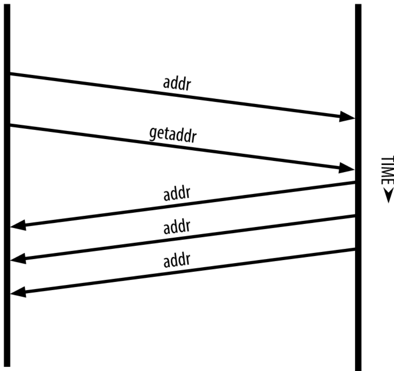
Figure 50. Address propagation and discovery
