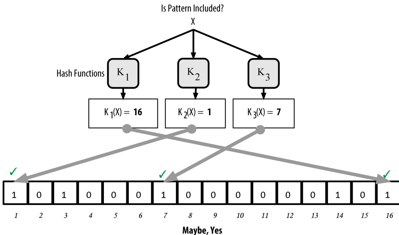
Figure 56. Testing the existence of pattern "X" in the bloom filter. The result is a probabilistic positive match, meaning "Maybe."
