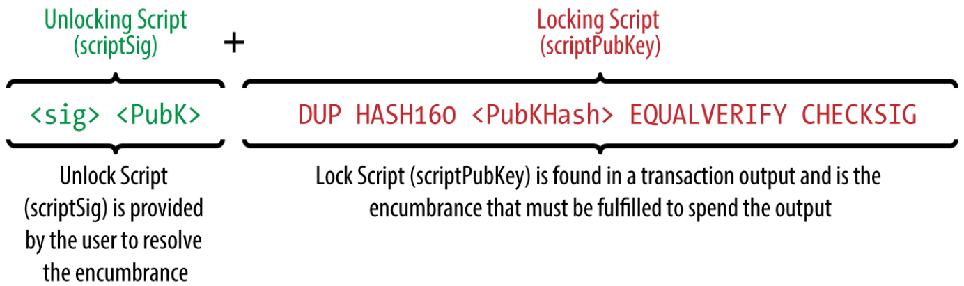
Figure 38. Combining scriptSig and scriptPubKey to evaluate a transaction script
