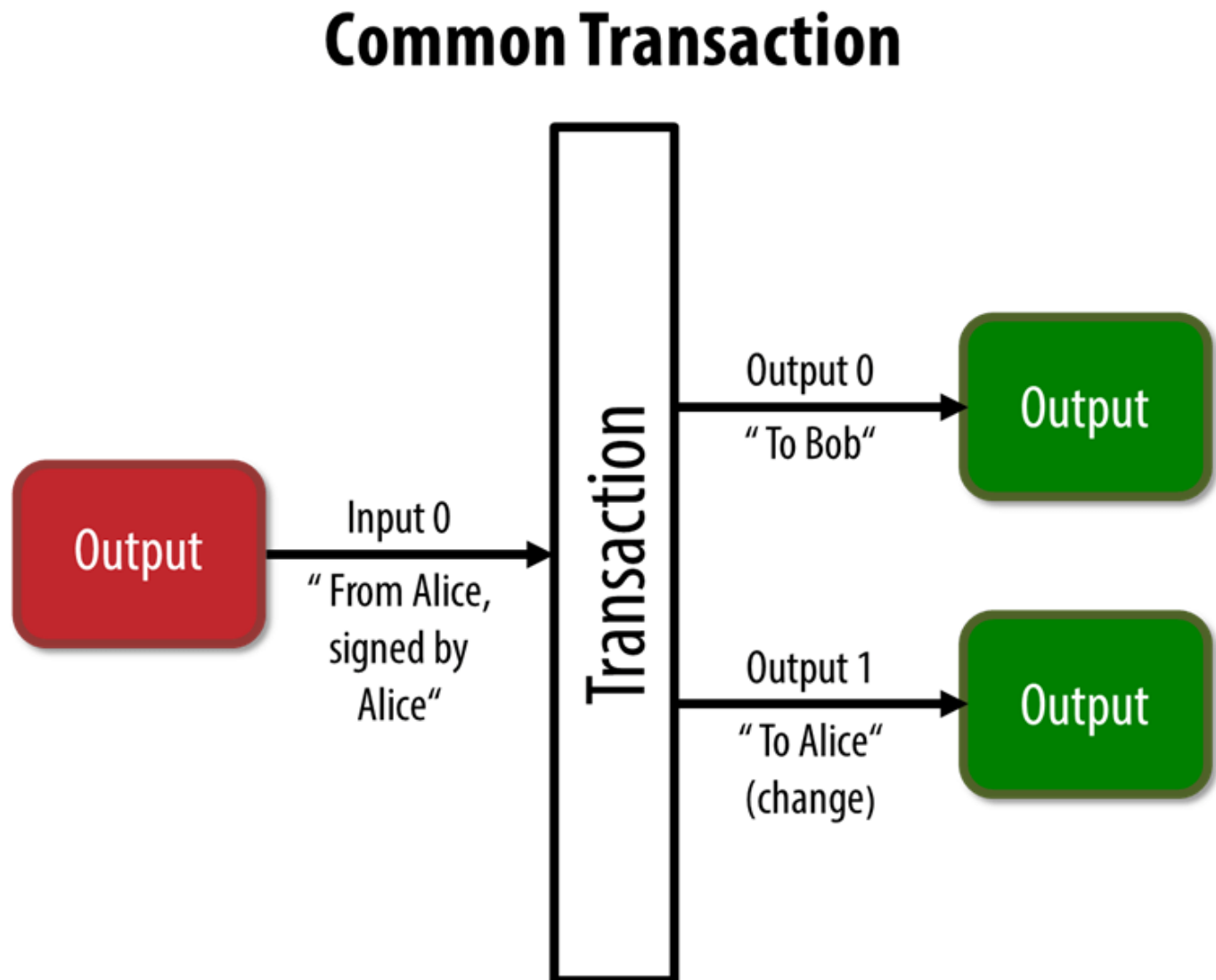
Figure 7. Most common transaction
