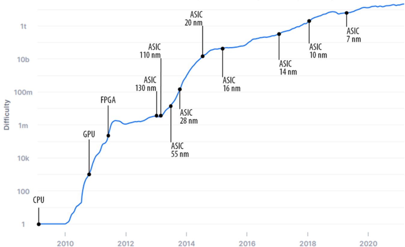
Figure 70. Bitcoin's mining difficulty metric (chart on a logarithmic scale)
