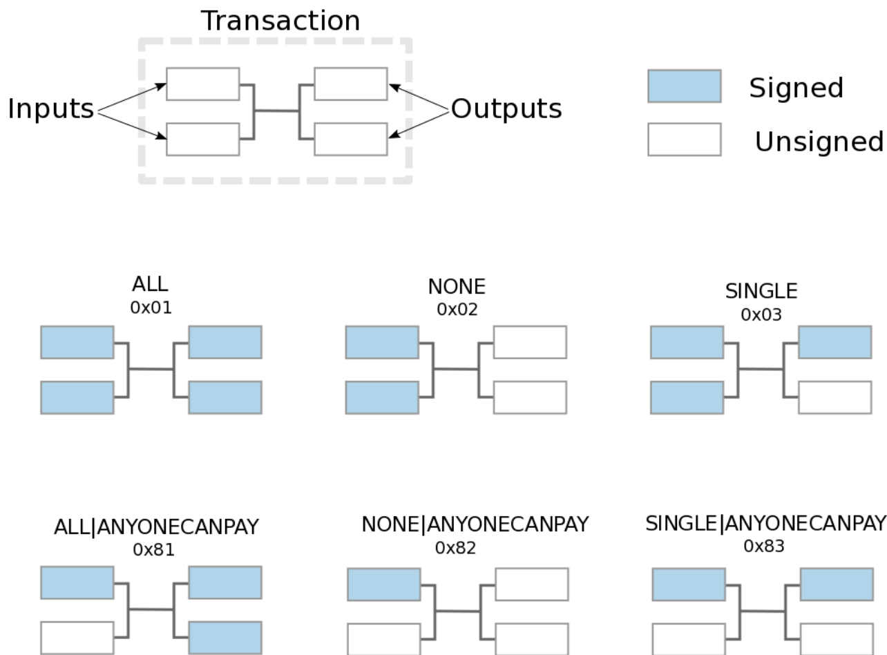
Figure 42. Summary of different sighash combinations
