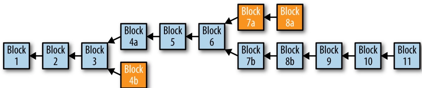
Figure 71. A blockchain with forks
