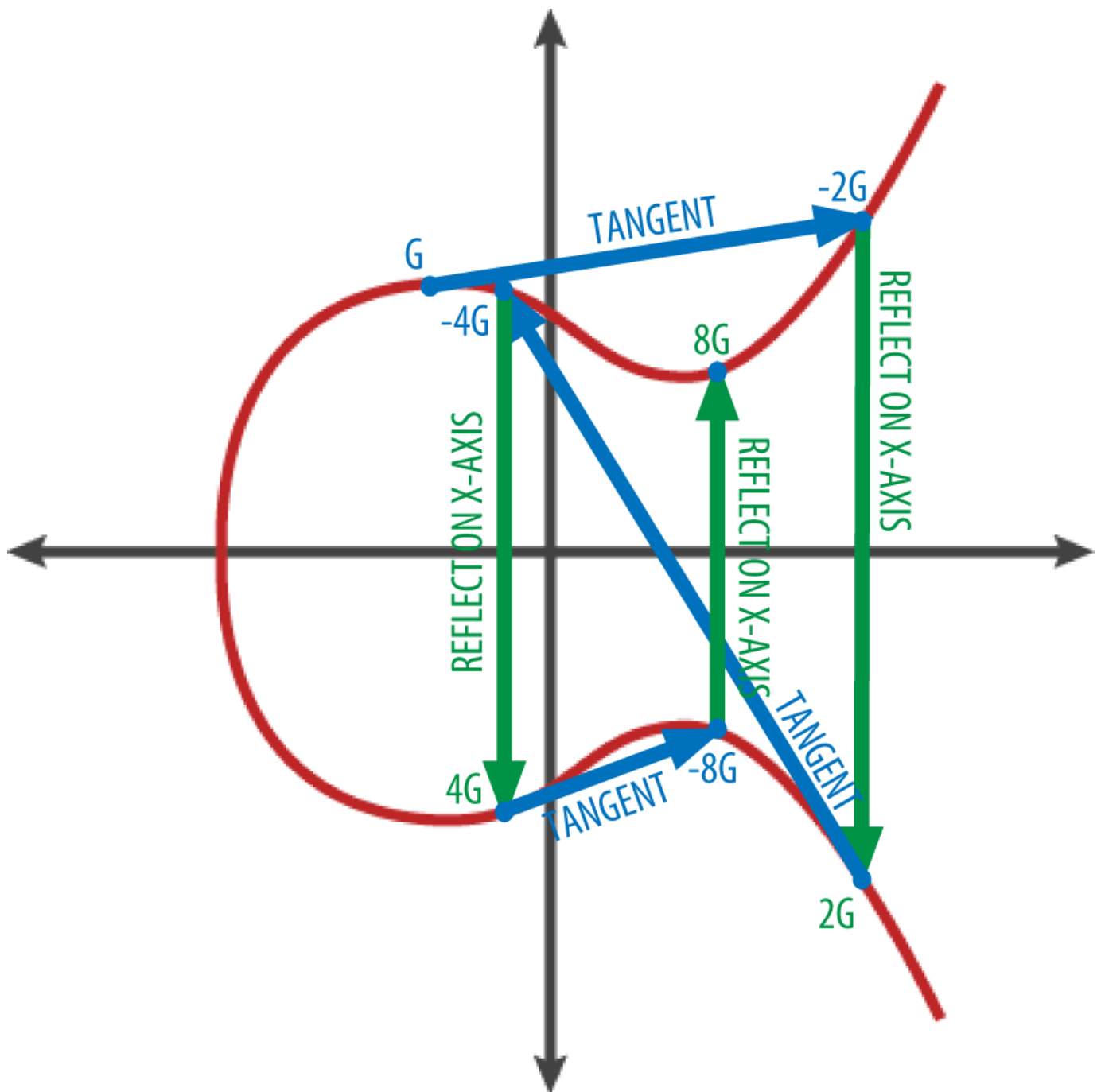
Figure 17. Elliptic curve cryptography: visualizing the multiplication of a point G by an integer k on an elliptic curve
