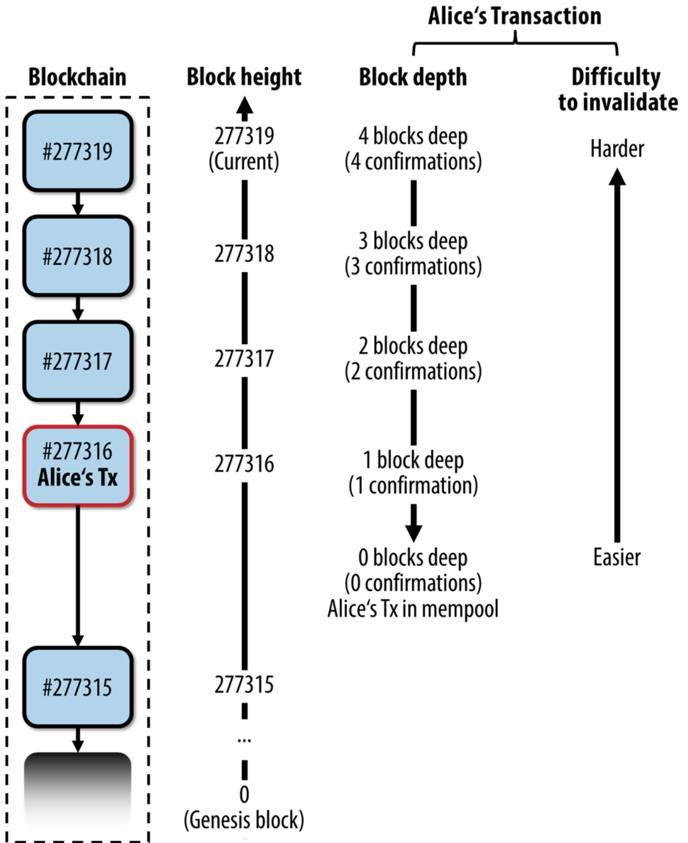
Figure 11. Alice's transaction included in block #277316
