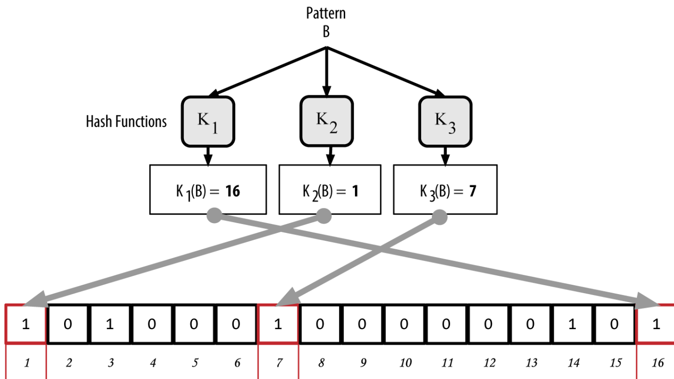
Figure 55. Adding a second pattern "B" to our simple bloom filter
