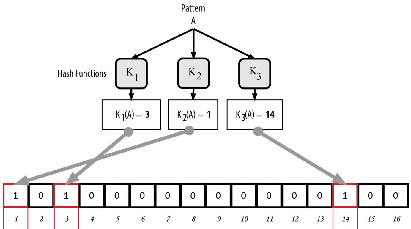
Figure 54. Adding a pattern "A" to our simple bloom filter
