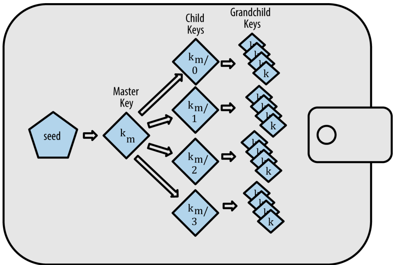
Figure 25. Type-2 HD wallet: a tree of keys generated from a single seed
