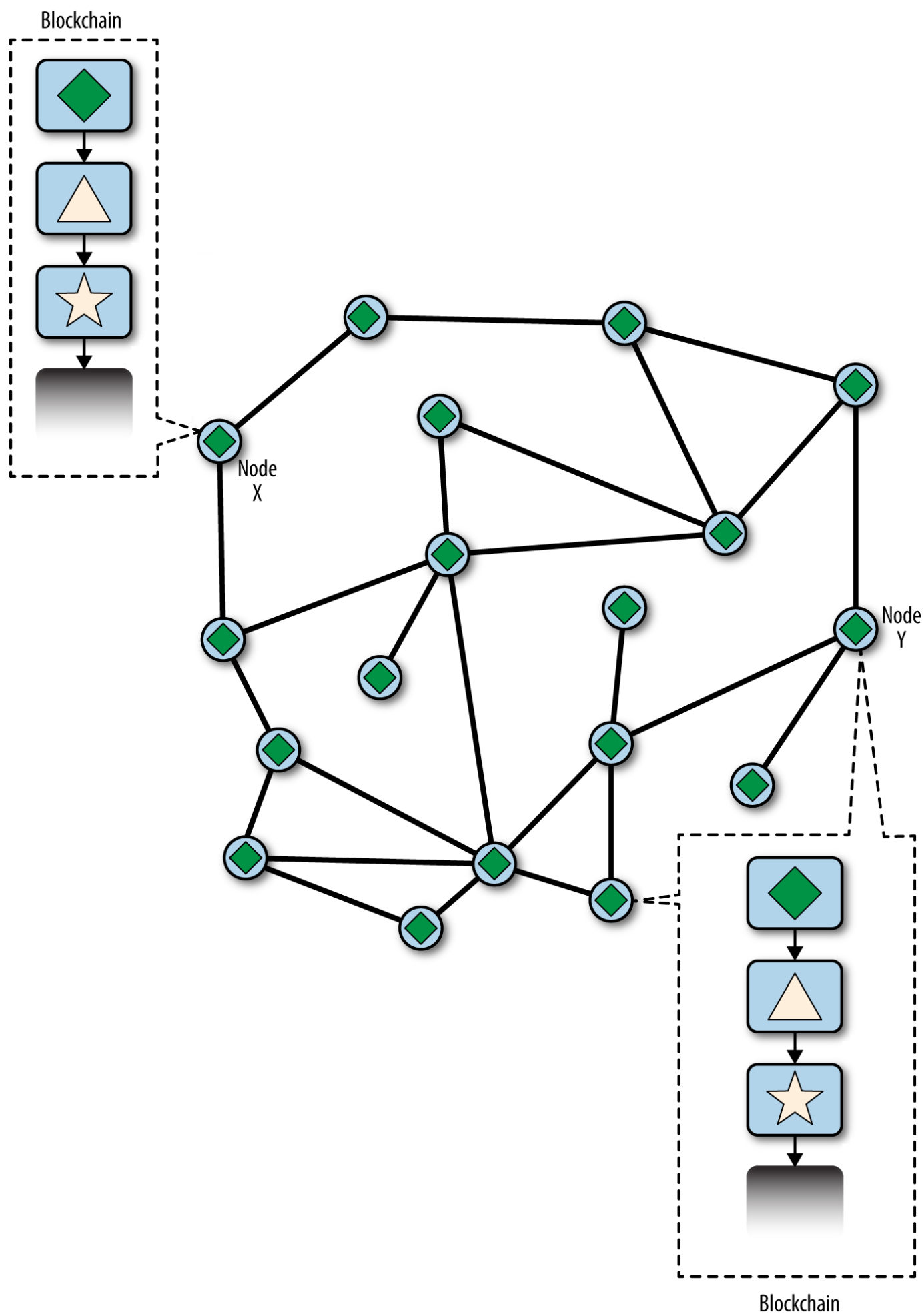
Figure 68. Visualization of a blockchain fork event: the network reconverges on a new longest chain
