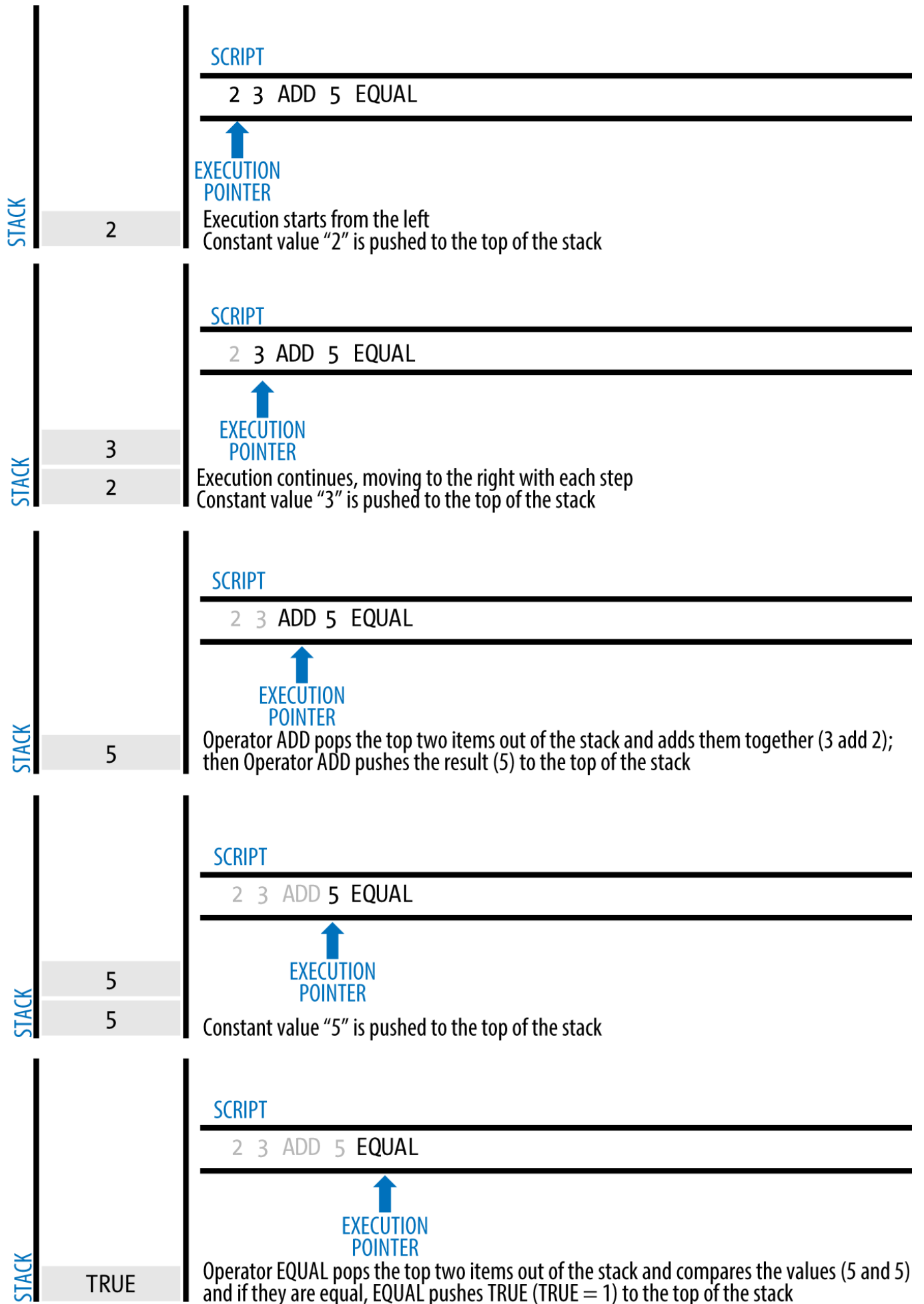
Figure 39. Bitcoin's script validation doing simple math
