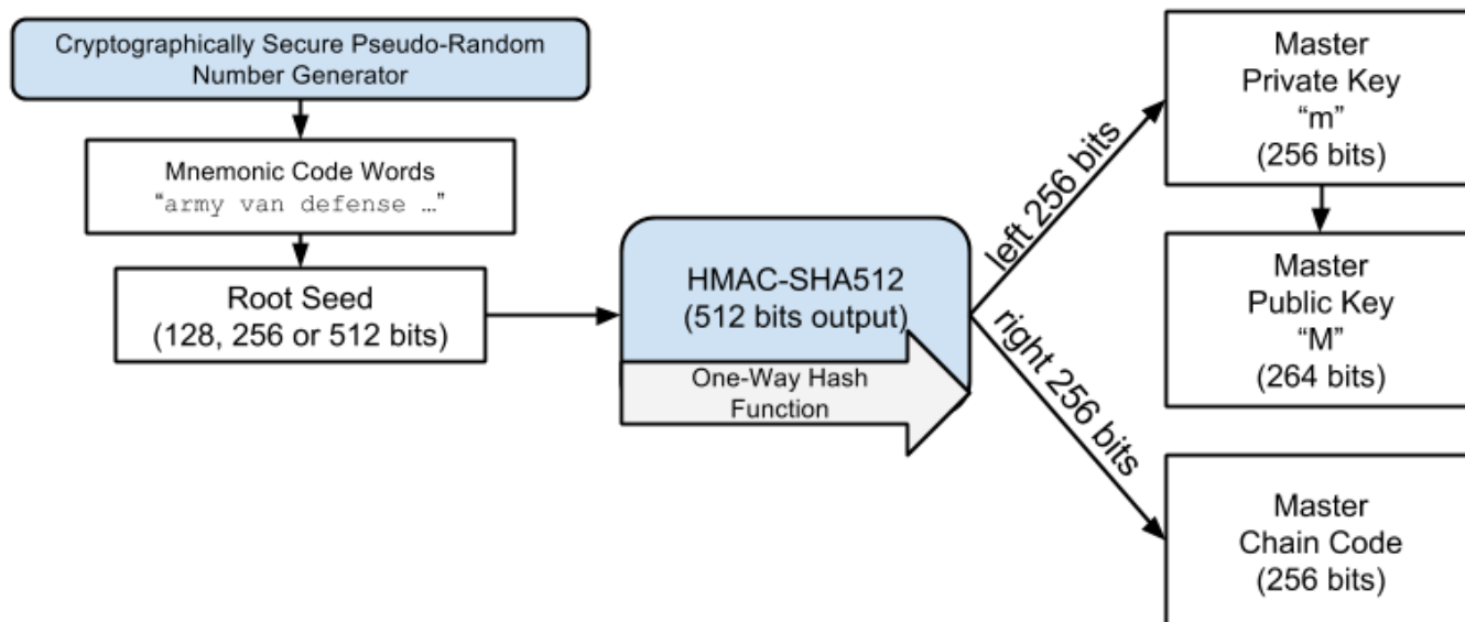
Figure 30. Creating master keys and chain code from a root seed
