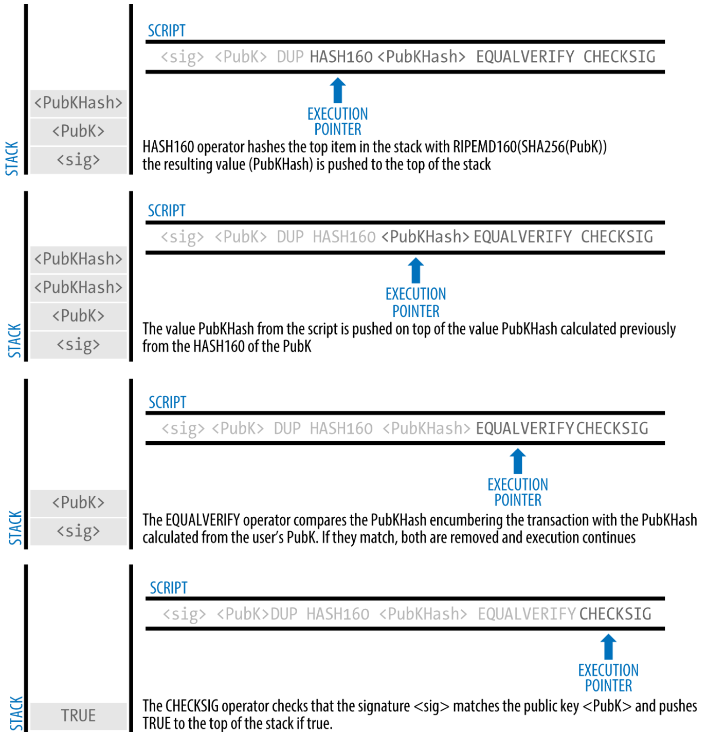
Figure 41. Evaluating a script for a P2PKH transaction (part 2 of 2)
