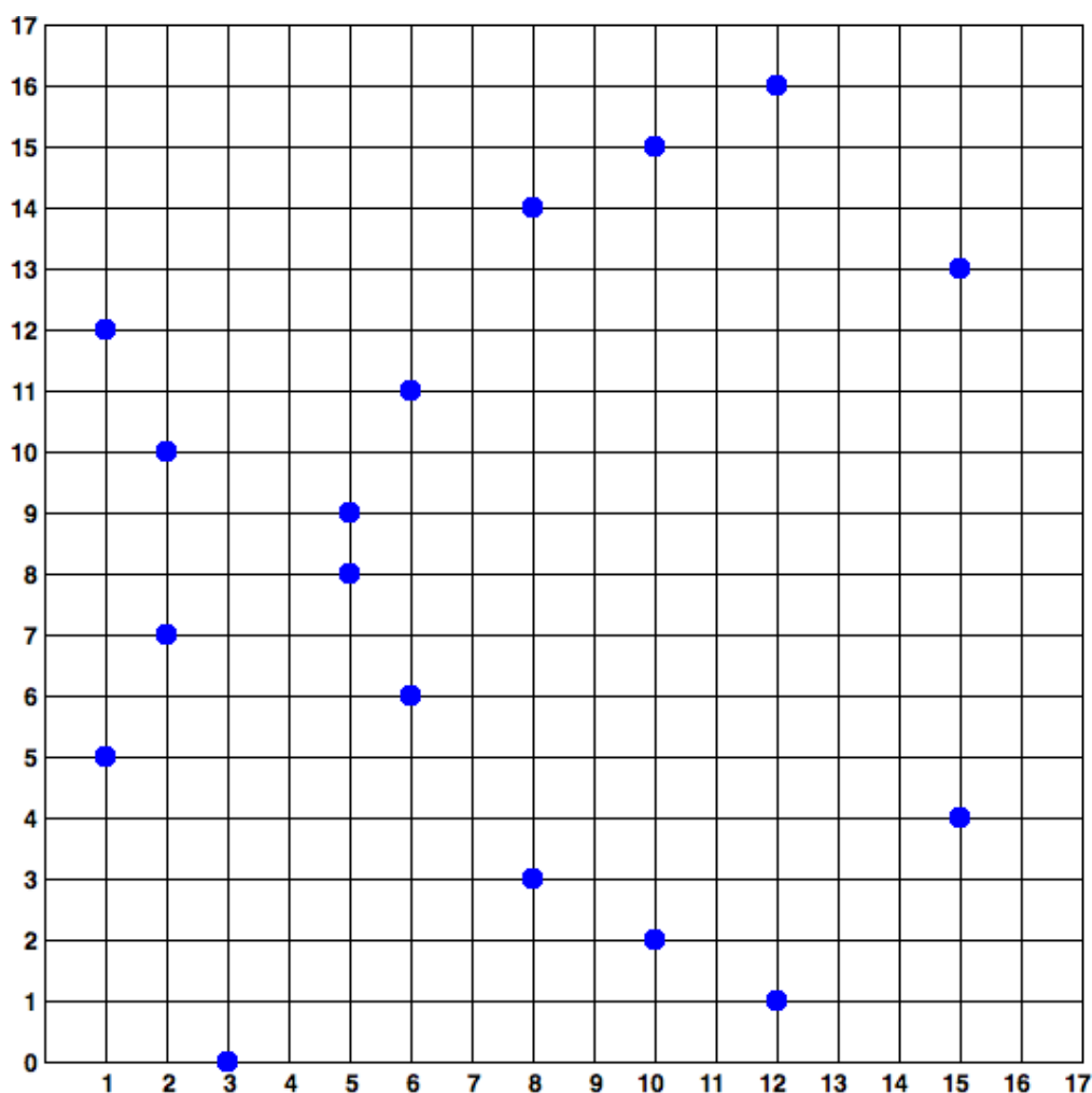
Figure 16. Elliptic curve cryptography: visualizing an elliptic curve over \mathbb{F}(p) , with p=17
