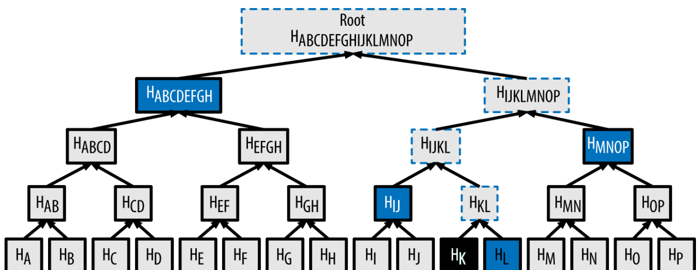
Figure 62. A merkle path used to prove inclusion of a data element
