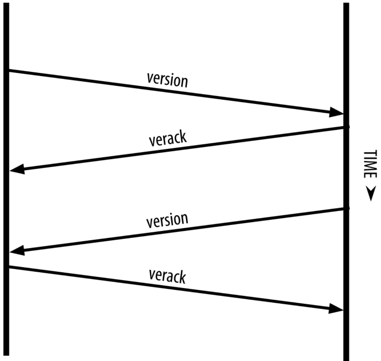
Figure 49. The initial handshake between peers
