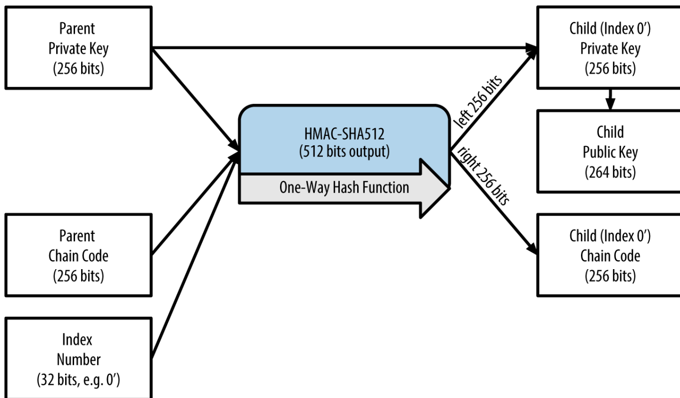
Figure 33. Hardened derivation of a child key; omits the parent public key
