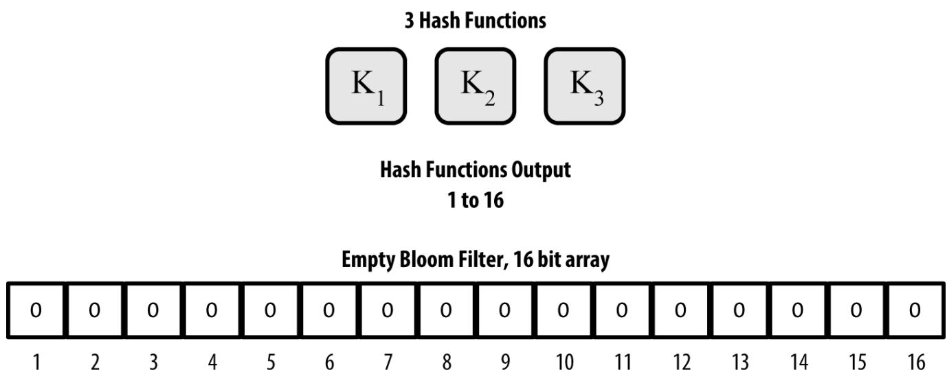
Figure 53. An example of a simplistic bloom filter, with a 16-bit field and three hash functions
