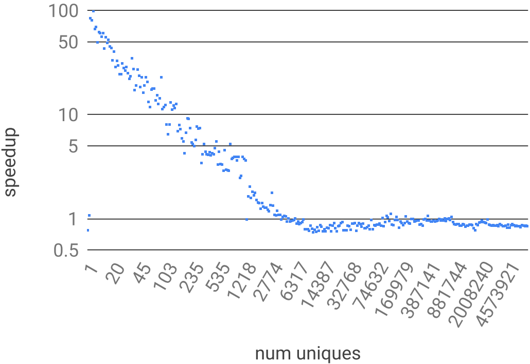
Fig. 12. Throughput speedup of eager ( \epsilon = 0.04 ) vs. no-eager ( \epsilon = 1.0 ) propagation, k = 4,096 .
