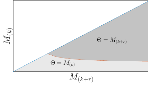
Fig. 7. Areas of M_{(k)} and M_{(k+r)} . In the dark gray \mathcal{A}_s induces \Theta = M_{(k+r)} , and in the light gray, \Theta = M_{(k)} . The white area is not feasible.
