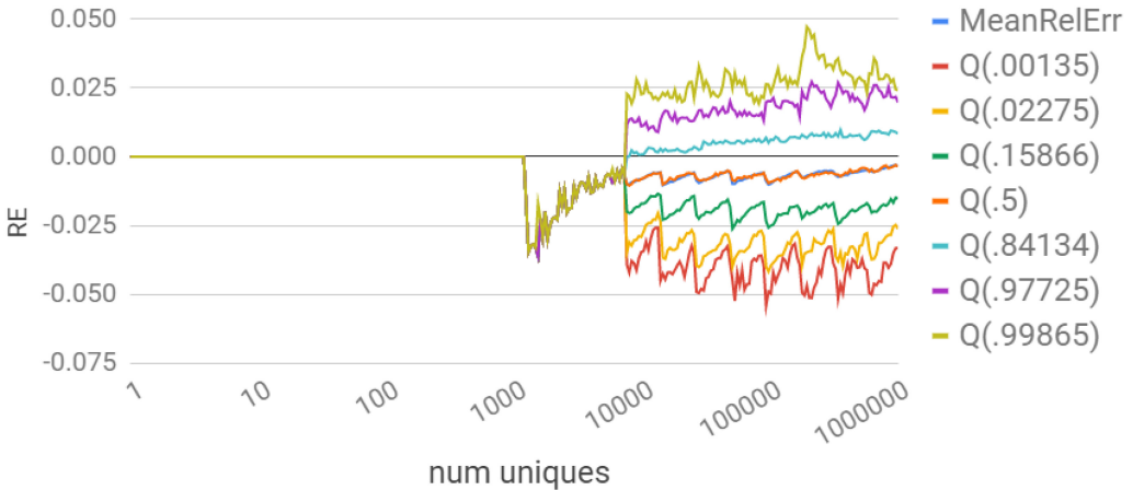
(b) With eager propagation, error bound defined by \epsilon = 0.04
