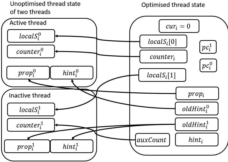
Fig. 6. Reference mapping of g when cur_i equals 0 before executing line 227.
