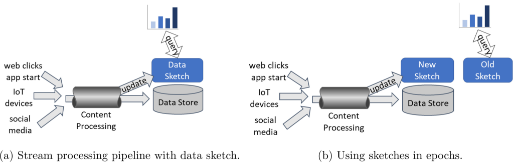
Fig. 1. Stream processing architectures.
