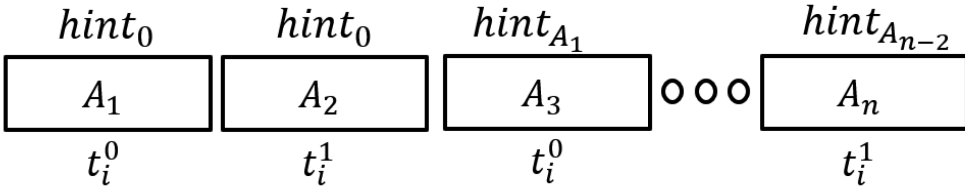
Fig. 5. Simulation of processing A = A_1 || A_2 || \dots || A_n .
