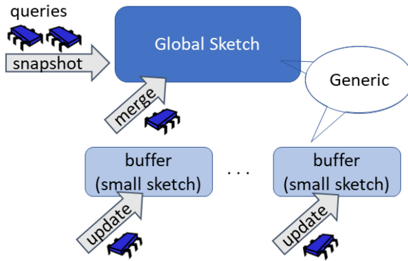
Fig. 2. Concurrent sketches architecture.
