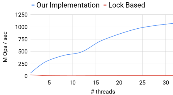
Fig. 3. Scalability of DataSketches’ \Theta sketch protected by a lock vs. our concurrent implementation.
