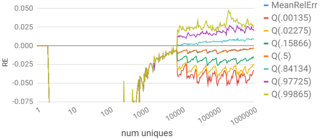
(a) No eager propagation ( \epsilon = 1.0 )
