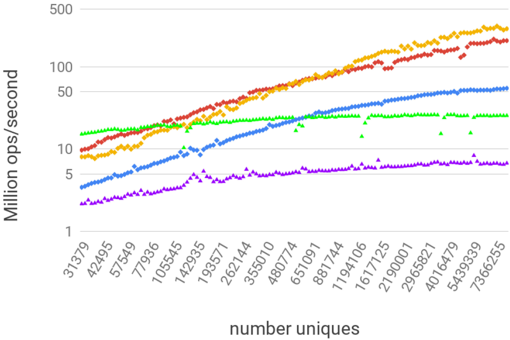
(b) Zooming-in on large sketches
