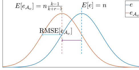
Fig. 8. Distribution of estimators e and e_{\mathcal{A}_w} . The RSE of e_{\mathcal{A}_w} with regards to n is bounded by the relative bias plus the RMSE of e_{\mathcal{A}_w} .
