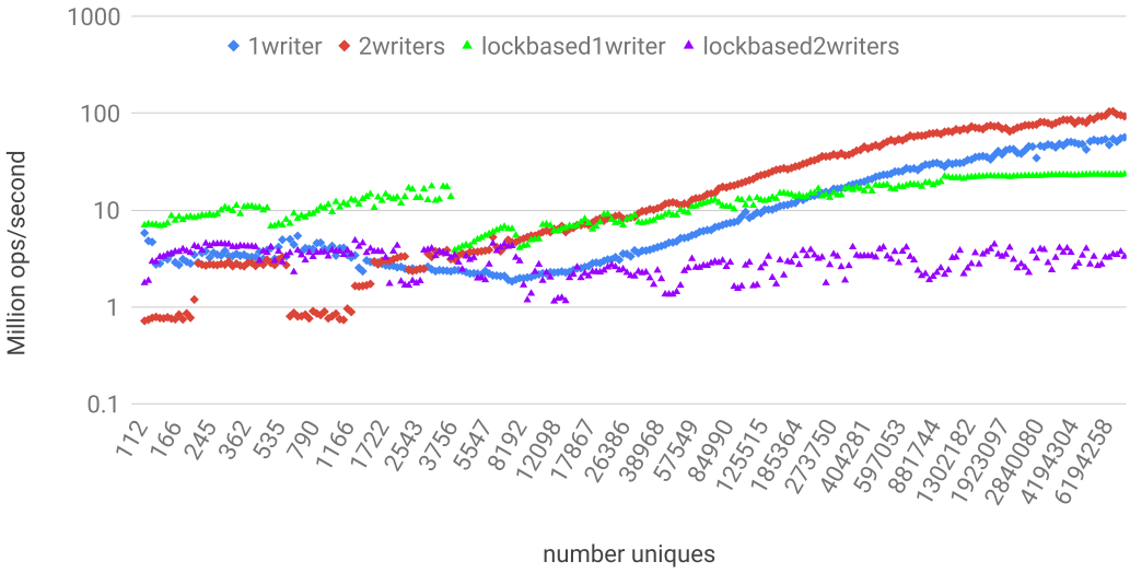
Fig. 11. Mixed workloads: writers with background reads, k = 4,096 , \epsilon = 0.04 .
